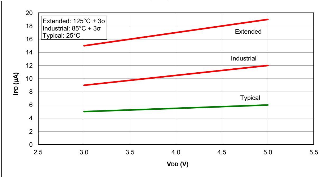
FIGURE 23-18: I PD , BROWN-OUT RESET (BOR), PIC16F753 ONLY
