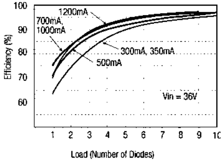
Efficiency/Load
