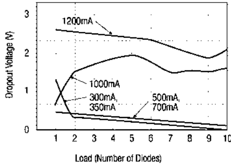
Dropout Voltage/Load
