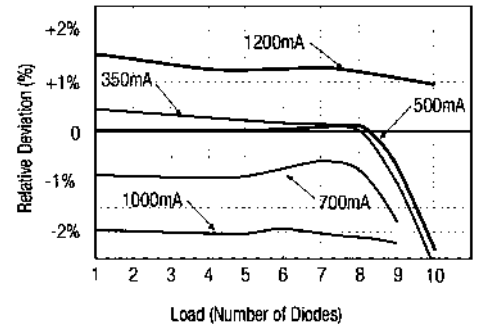
Output Current Accuracy/Load
