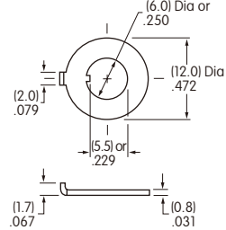
AT506M Locking Ring Steel with Zinc/Chrome
