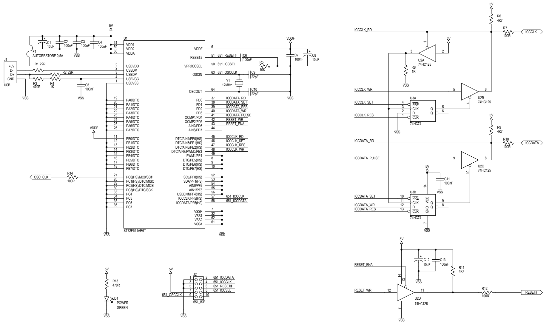
USB TO ICC INTERFACE
