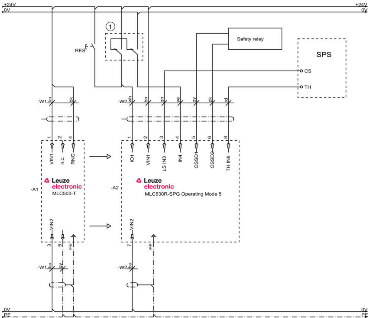
1 Optionaler Einlern-Schlüsseltaster
