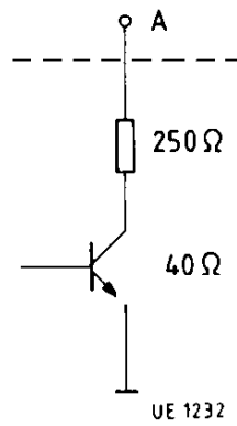
Internal Circuitry of an Output A:
