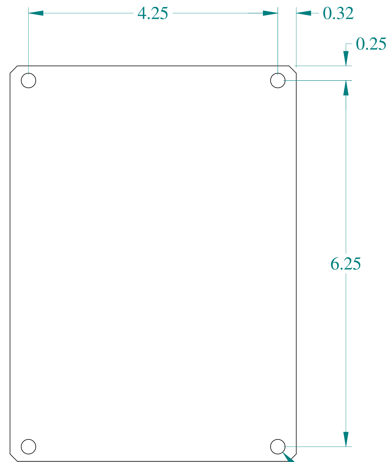
FRONT VIEW
