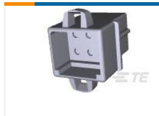
TE Part #1-480276-0 06P CMNL CAP HSG P/M NATL
