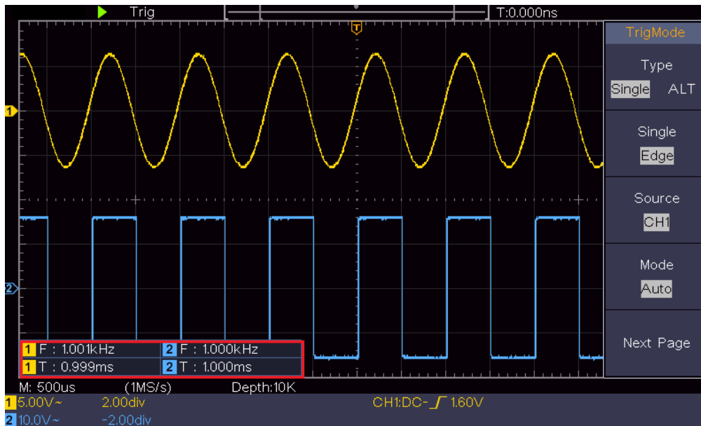
Figure 0-6 Automatic measurement
