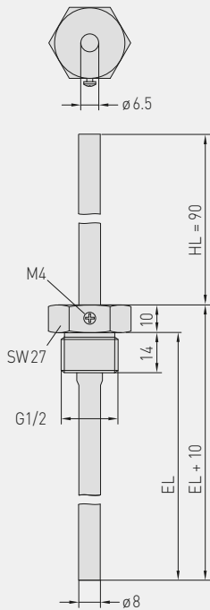
Dimensional drawing TH- VA / xx / 90
