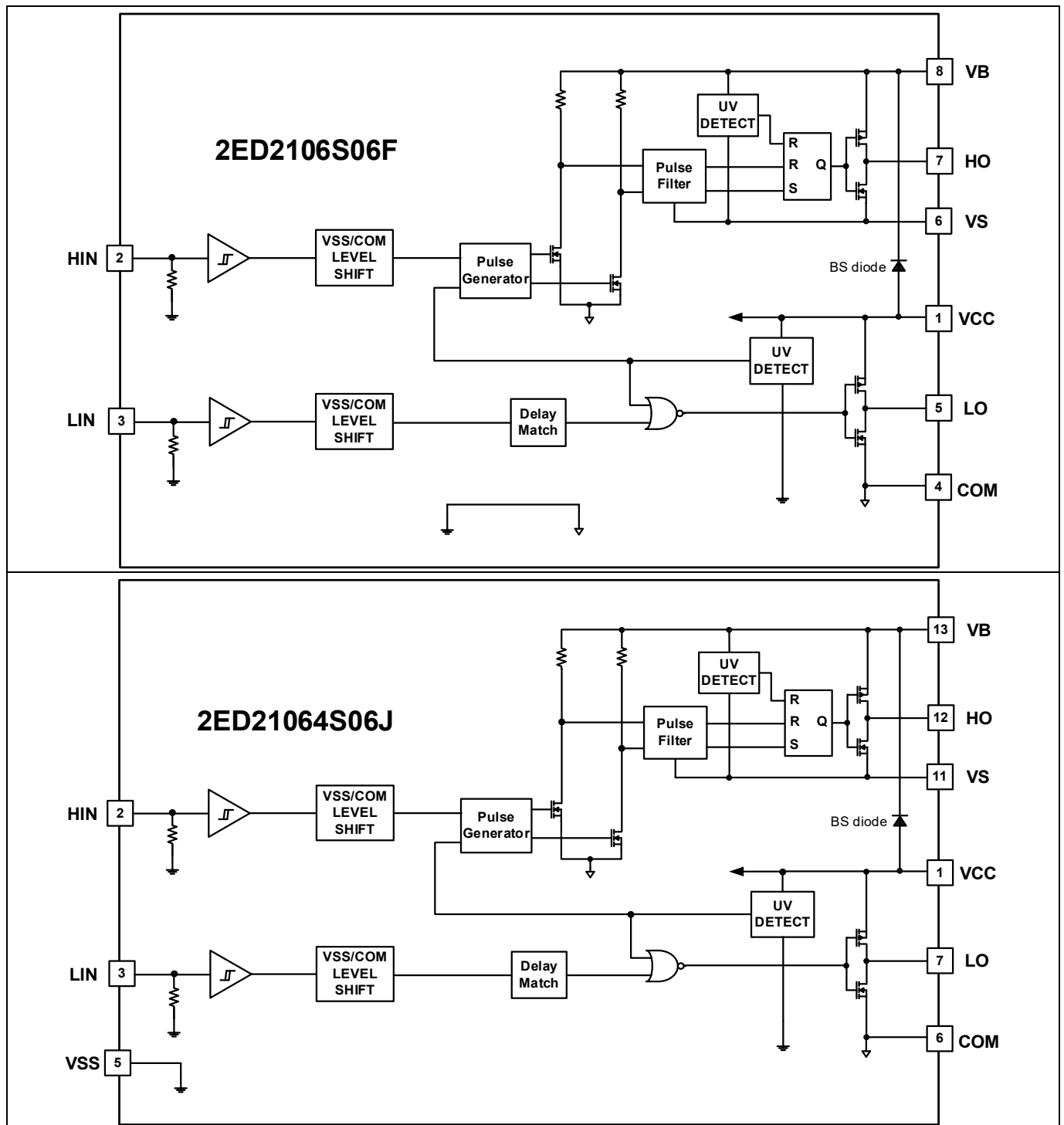
Figure 2 Block diagrams
