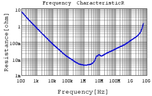
GRM188R6YA475KE15 R DCOV, 25degC
