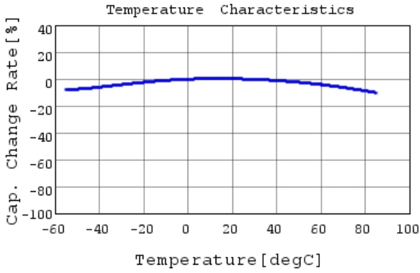
GRM188R6YA475KE15 C-Temp. capchange, DC0.0V,
