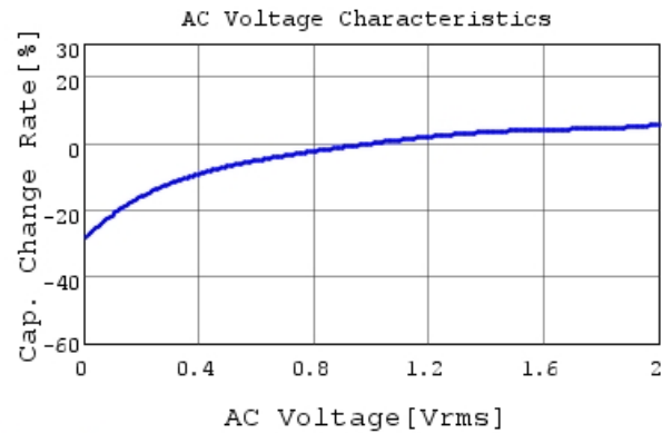
GRM188R6YA475KE15 C-AC Voltage capchange, Dc
