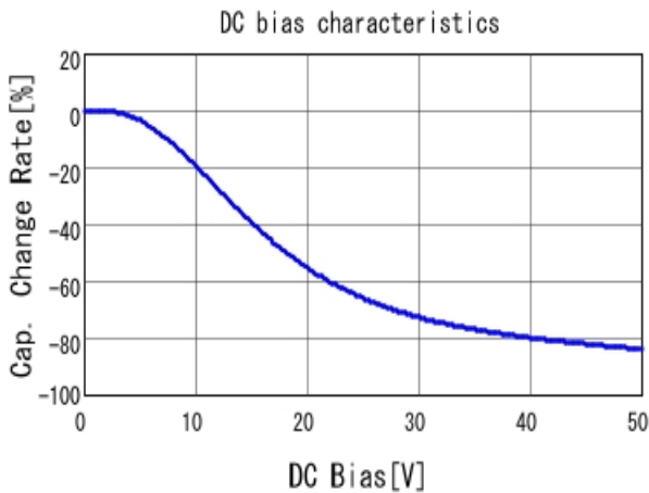
GCM155L8EH104KE07 C-DC bias capchange, 25.0degC, AC1.
