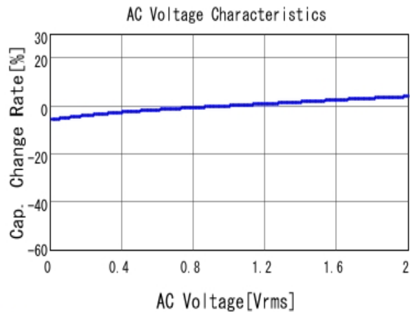
GCM155L8EH104KE07 C-AC Voltage capchange, DCOV, 25.0d
