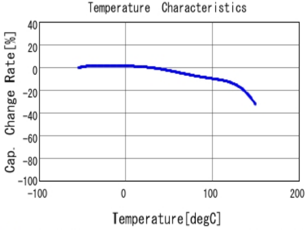
GCM155L8EH104KE07 C-Temp. capchange, DC0.0V, AC1.0V rm
