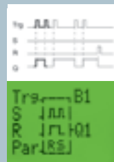
Stromstoß-relais
