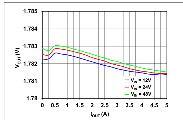
FIGURE 2-6: Output Voltage vs. Output Current ( V_{OUT} = 1.8V ).
