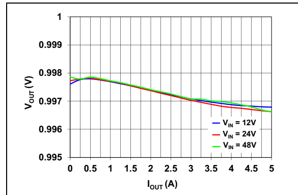
FIGURE 2-5: Output Voltage vs. Output Current ( V_{OUT} = 1V ).
