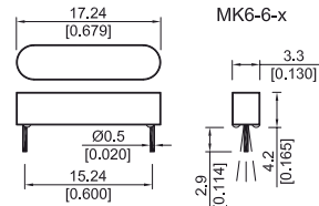
Angle of pins may deviate \pm 7.5^\circ
