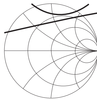
Figure 21. Load and Source Stability Circles.
