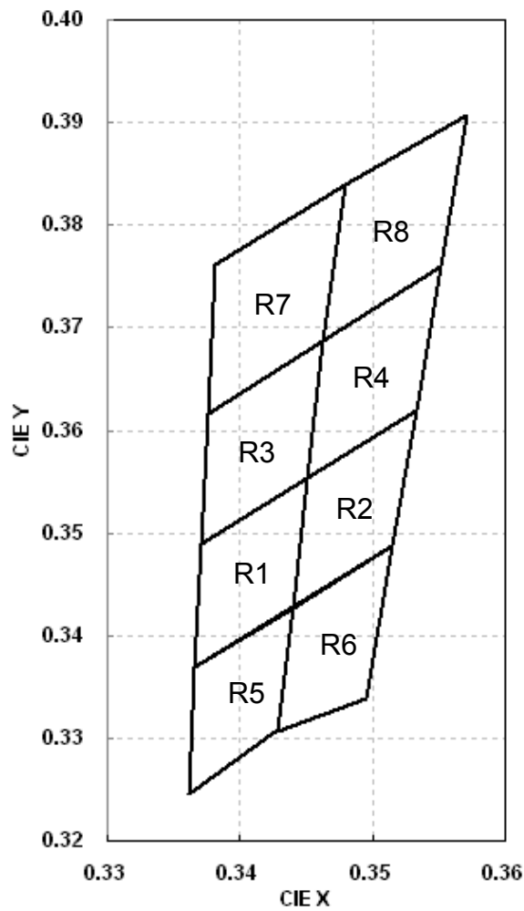
CIE Diagram
