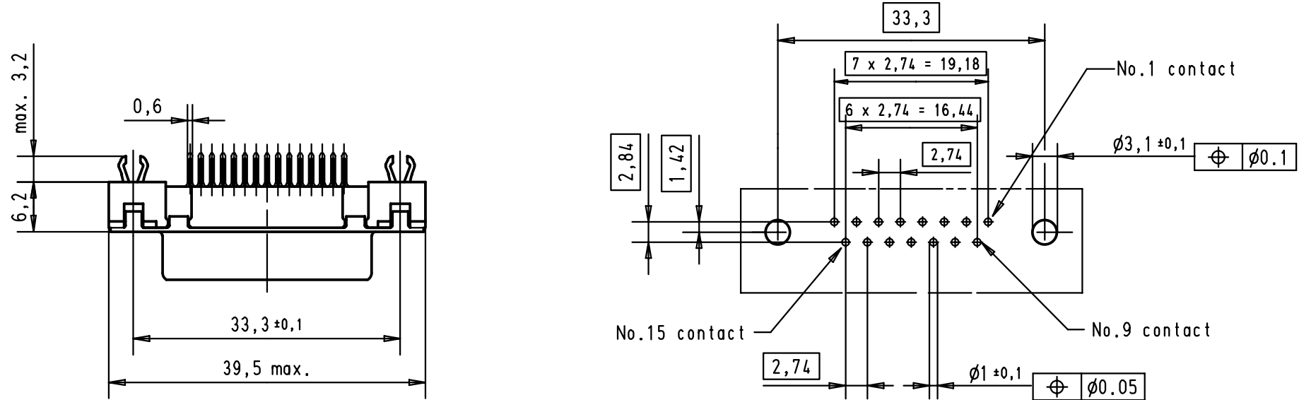
Printed board layout component side
