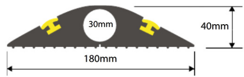
Type TTC/2
