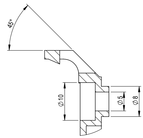
DETAIL Z SCALE 2 : 1
