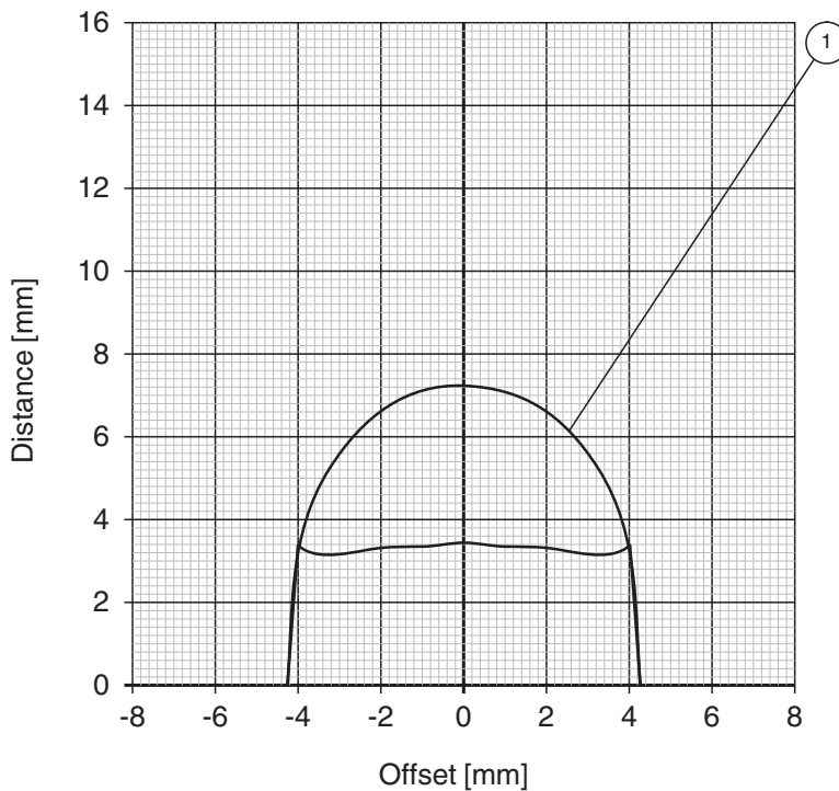
Reading range in steel IQC21-8
