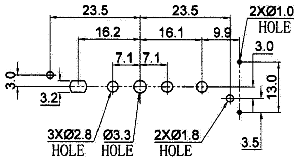
PCB/MOUNTING LAYOUT
