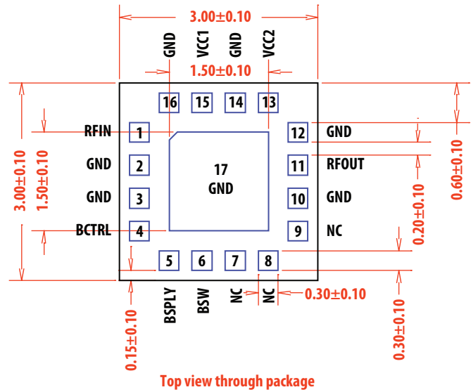
Figure 34. Package dimensions
