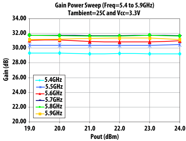
Figure 9. Gain Power Sweep at Vcc=3.3V and 25C over Frequency
