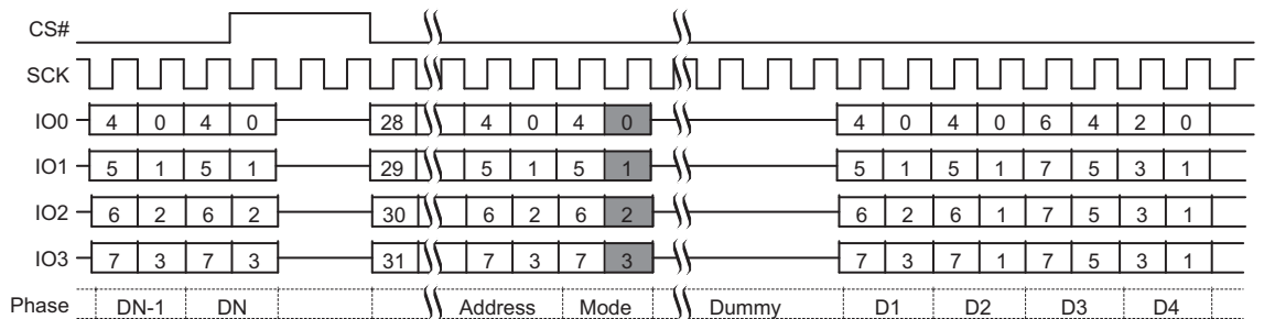
Figure 10.36 Continuous Quad I/O Read Command Sequence (4-Byte Address)
