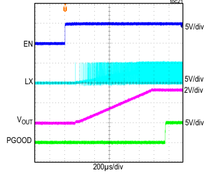
MAXM17624 STARTUP THROUGH ENABLE ( V_{IN} = 5V , V_{OUT} = 3.3V , I_{LOAD} = 0A , PWM MODE)
