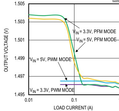
MAXM17623 OUTPUT VOLTAGE vs. LOAD CURRENT ( V_{OUT} = 1.5V , PWM AND PFM MODE)
