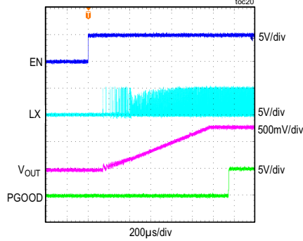
MAXM17623 STARTUP THROUGH ENABLE ( V_{IN} = 5V , V_{OUT} = 0.8V , I_{LOAD} = 1A , PWM MODE)
