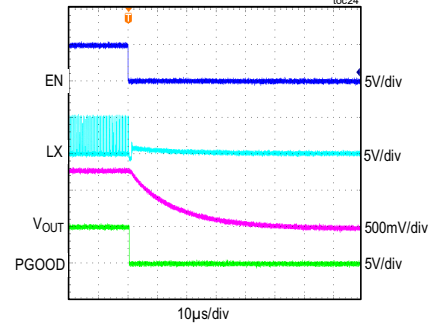
MAXM17623 SHUTDOWN THROUGH ENABLE ( V_{IN} = 5V , V_{OUT} = 0.8V , I_{LOAD} = 1A , PWM MODE)
