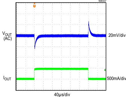
MAXM17623 LOAD TRANSIENT RESPONSE ( V_{IN} = 3.3V , V_{OUT} = 0.8V , PWM MODE) (LOAD CURRENT STEPPED FROM 0A TO 0.5A)
