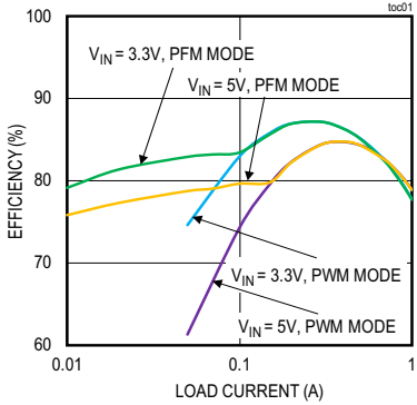
MAXM17623 EFFICIENCY vs. LOAD CURRENT ( V_{OUT} = 0.8V , PWM AND PFM MODE)
