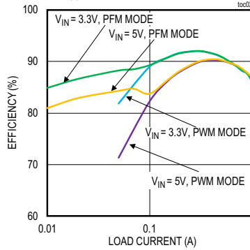
MAXM17623 EFFICIENCY vs. LOAD CURRENT ( V_{OUT} = 1.5V , PWM AND PFM MODE)
