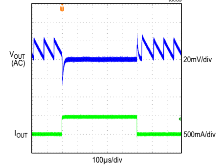
MAXM17623 LOAD TRANSIENT RESPONSE ( V_{IN} = 3.3V , V_{OUT} = 0.8V , PFM MODE) (LOAD CURRENT STEPPED FROM 0A TO 0.5A)
