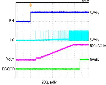
MAXM17623 STARTUP THROUGH ENABLE ( V_{IN} = 5V , V_{OUT} = 0.8V , I_{LOAD} = 0A , PWM MODE)
