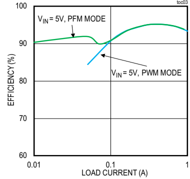
MAXM17624 EFFICIENCY vs. LOAD CURRENT ( V_{OUT} = 3.3V , PWM AND PFM MODE)
