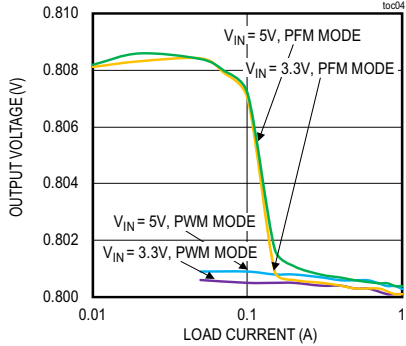
MAXM17623 OUTPUT VOLTAGE vs. LOAD CURRENT ( V_{OUT} = 0.8V , PWM AND PFM MODE)
