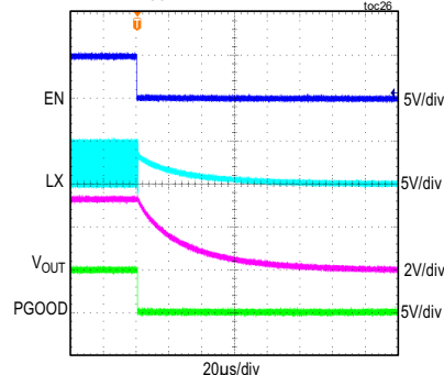
MAXM17624 SHUTDOWN THROUGH ENABLE ( V_{IN} = 5V , V_{OUT} = 3.3V , I_{LOAD} = 1A , PWM MODE)
