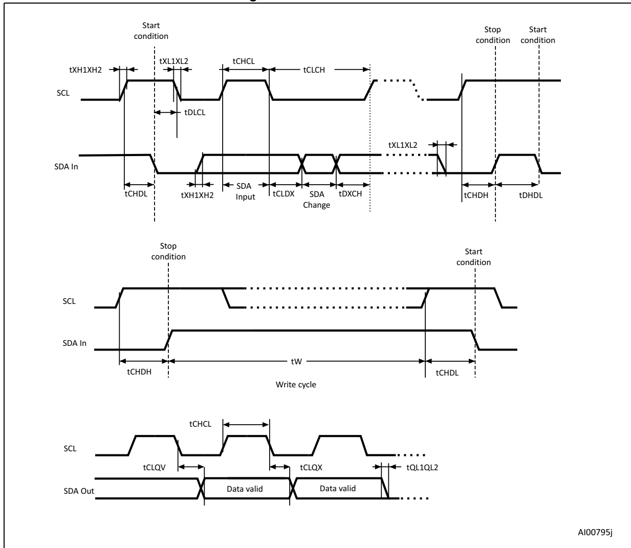
Figure 11. AC waveforms
