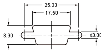
Panel Cutout
