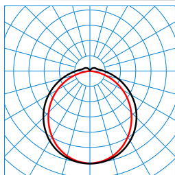
Deveo Fit 1500 4000-840 PC TX369762
