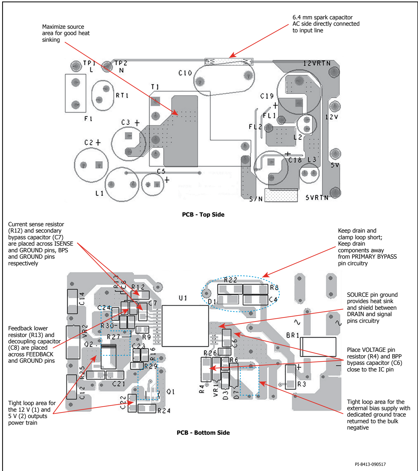
Figure 16. PCB.
