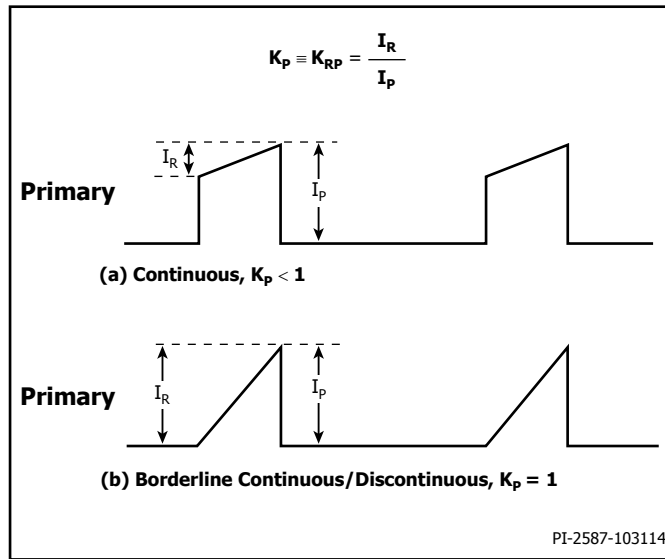
Figure 17. Continuous Mode Current Waveform, K_P \leq 1 .
