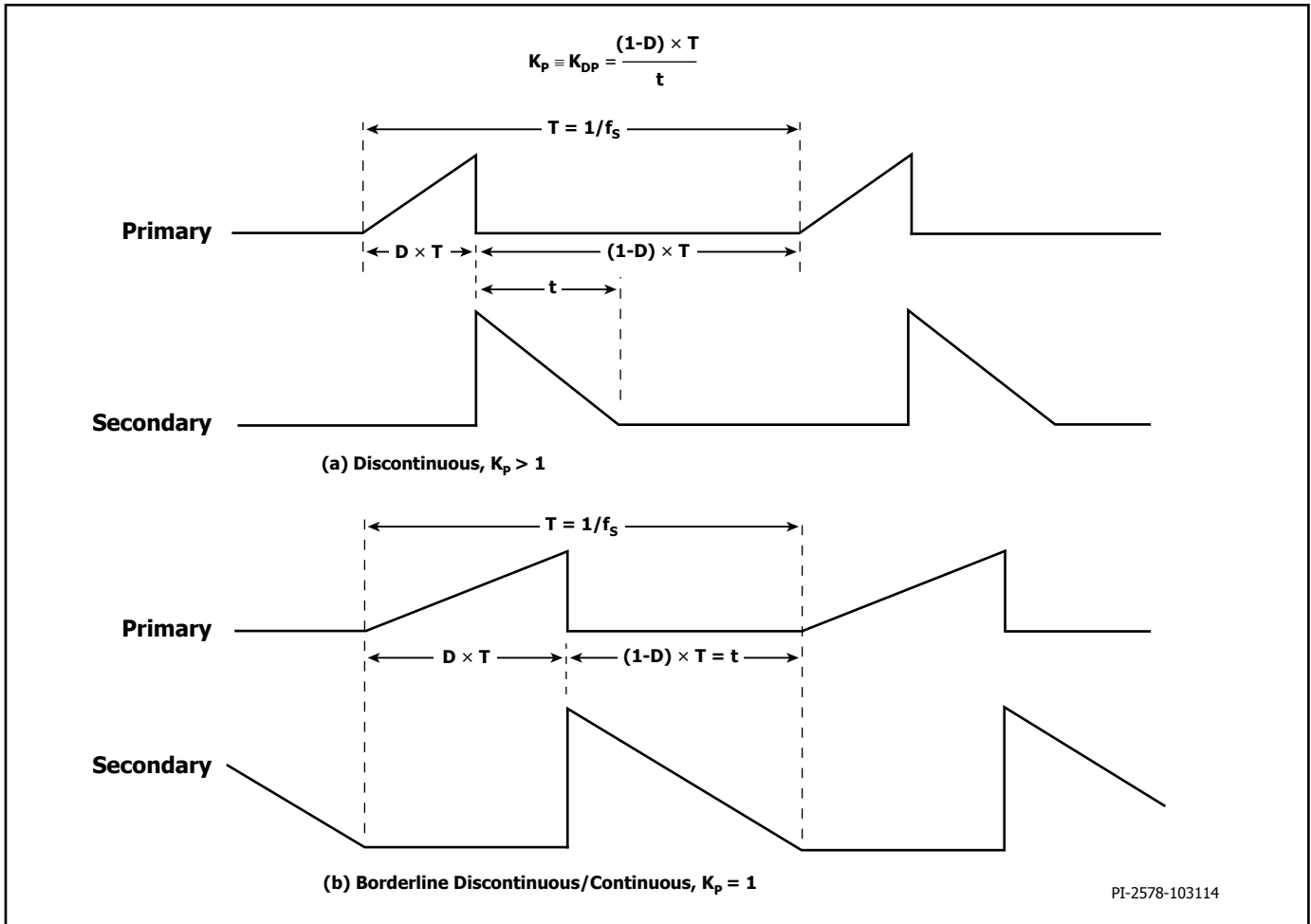
Figure 18. Discontinuous Mode Current Waveform, K_p \geq 1 .
