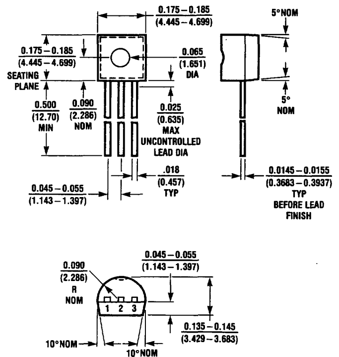
Z Package TO-92 Plastic
