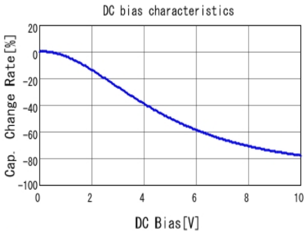
■ GRT155R71A474KE01 C-DC bias capchange, 25.0degC, AC1V
