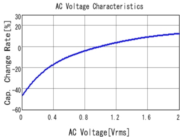
■ GRT155R71A474KE01 C-AC Voltage capchange, DCOV, 25.0d
