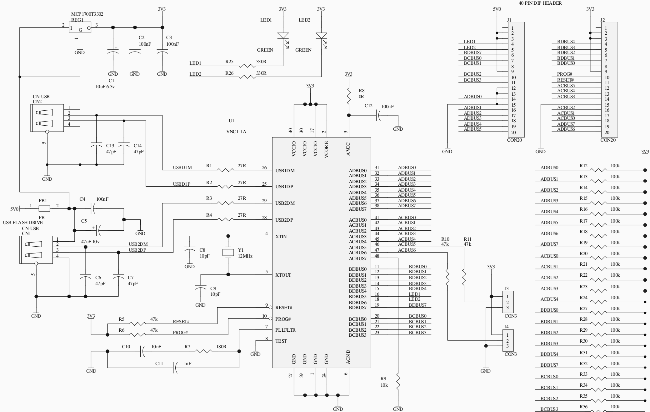
VINCLUM VDIP2 SCHEMATIC
