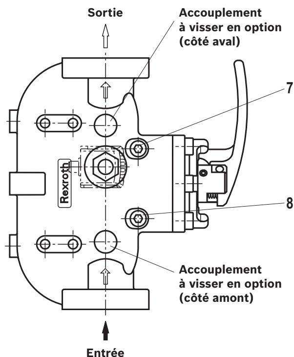
Type 50LDN0160
