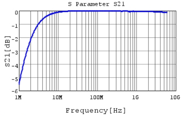
GRM1885C1H102JA01 S21 DCOV, 25degC
