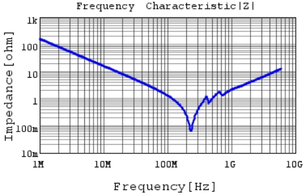
GRM1885C1H102JA01 |Z| DCOV, 25degC
