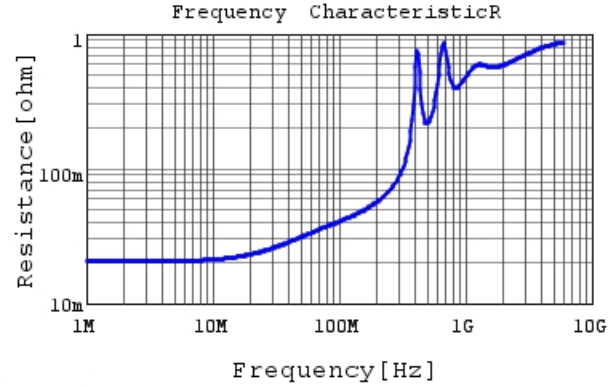
GRM1885C1H102JA01 R DCOV, 25degC
