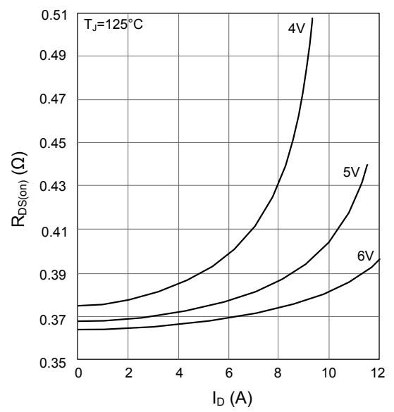
Figure 9. Typ R_{DS(on)\_LS} vs. I_D at T_J=125^\circ\text{C}
