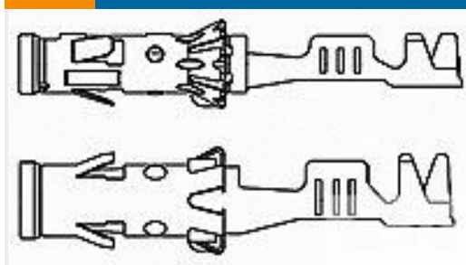
TE Part # 962981-1 2,5MMD SOCKET CONTACT
