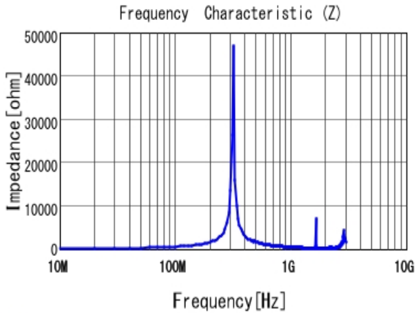
■ LQW2BASR82J00 |Z|
