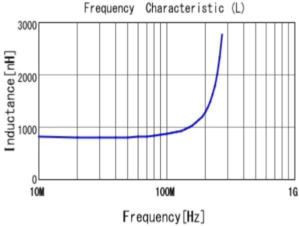
■ LQW2BASR82J00 L
