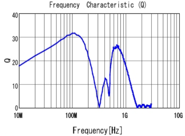
■ LQW2BASR82J00 Q
