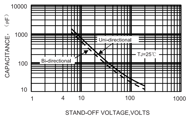
FIG.4-TYPICAL JUNCTION CAPACITANCE
