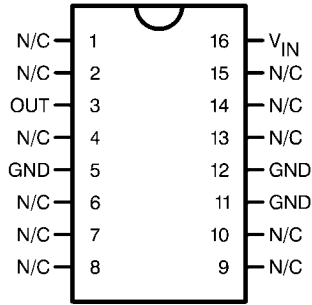
1208028 16-Lead Ceramic Surface-Mount Package (Top View) Order Part Number LM3940WG-3.3-QML 5962-9688401QXA NSC Drawing Number WG16A
