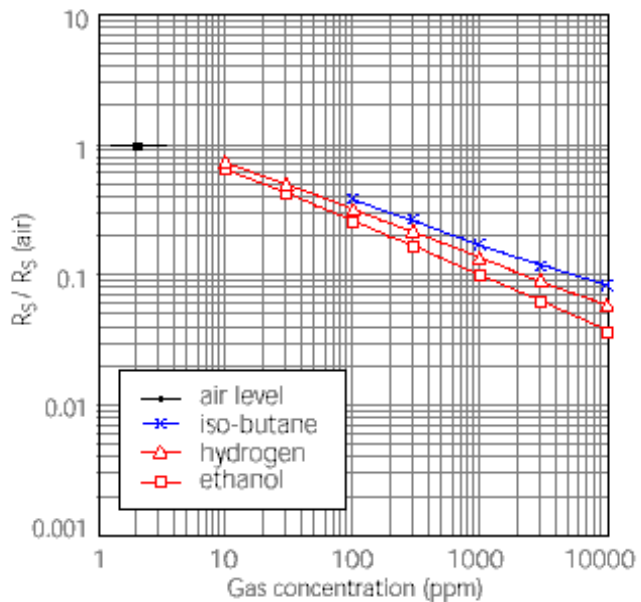
Fig 3. Sensitivity characteristics
