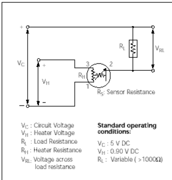
Fig 2. Standard circuit
