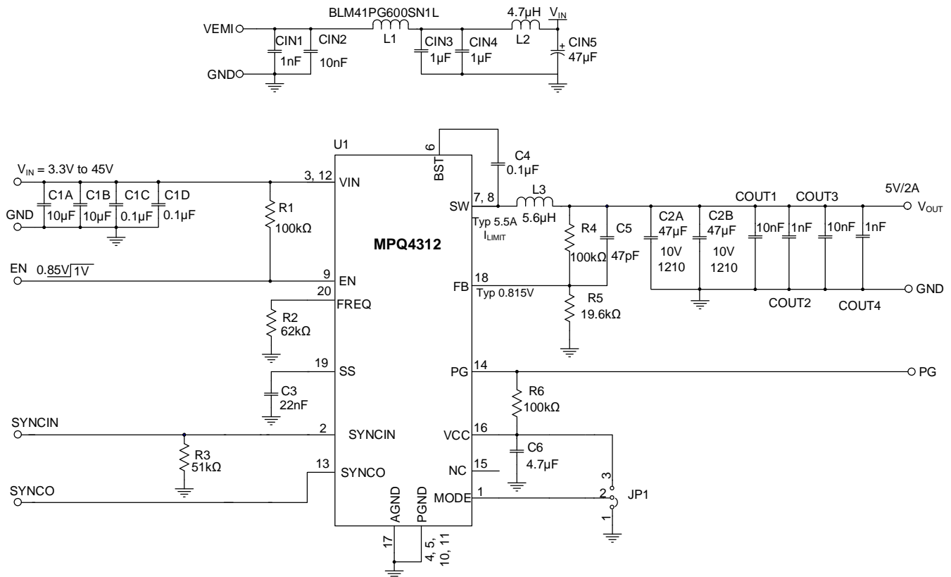
Figure 11: V OUT = 5V, f sw = 470kHz with EMI Filters
