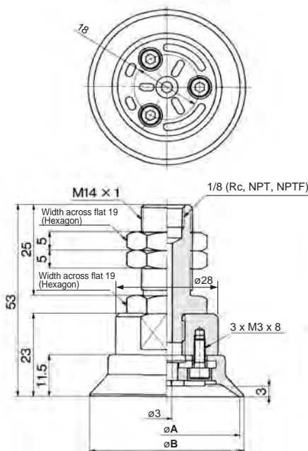
ZPT 40 50 H□-A14 (Male thread)
