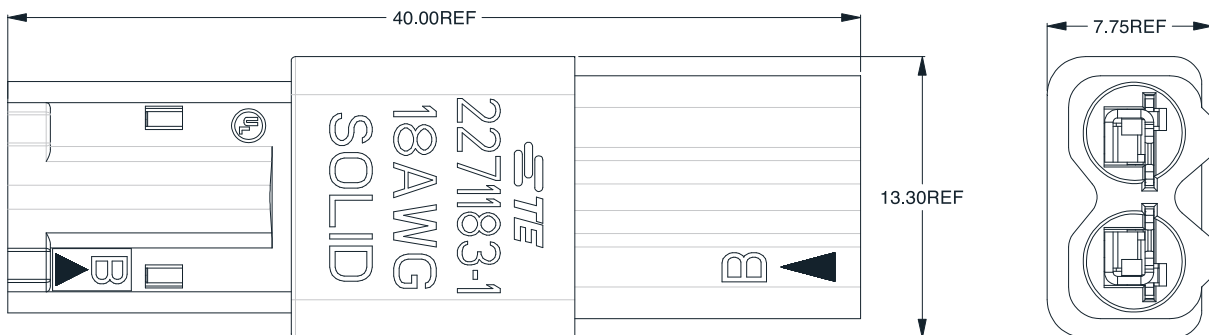
Mated Connector (2271203-1) :
