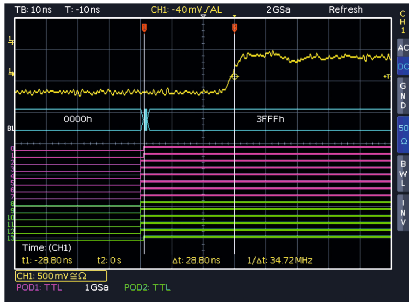
14 Bit DAC Signalwechsel
