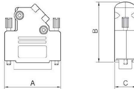
D-Sub-Hood
