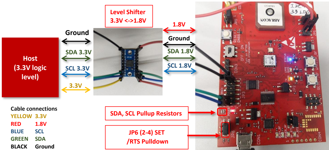
Figure 16: Erinome-II- GNSS evaluation board connection to 3.3V Host
