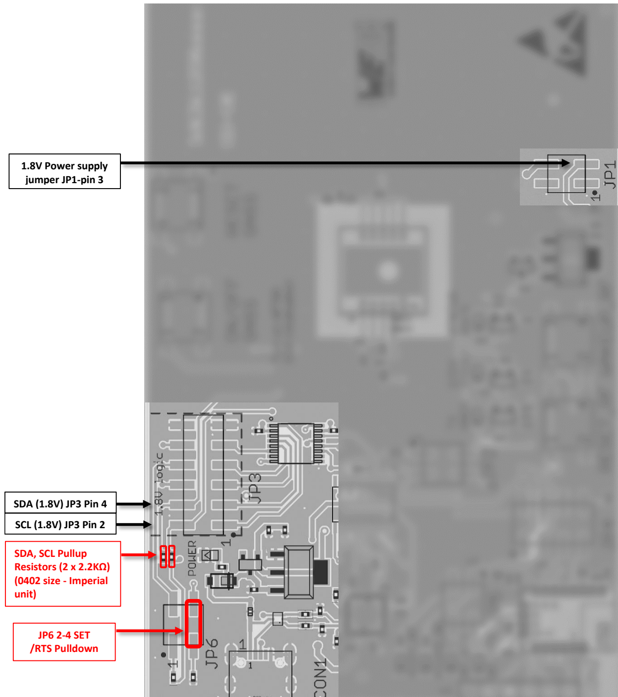
Figure 15: I 2 C evaluation board modification - Erinome-II
