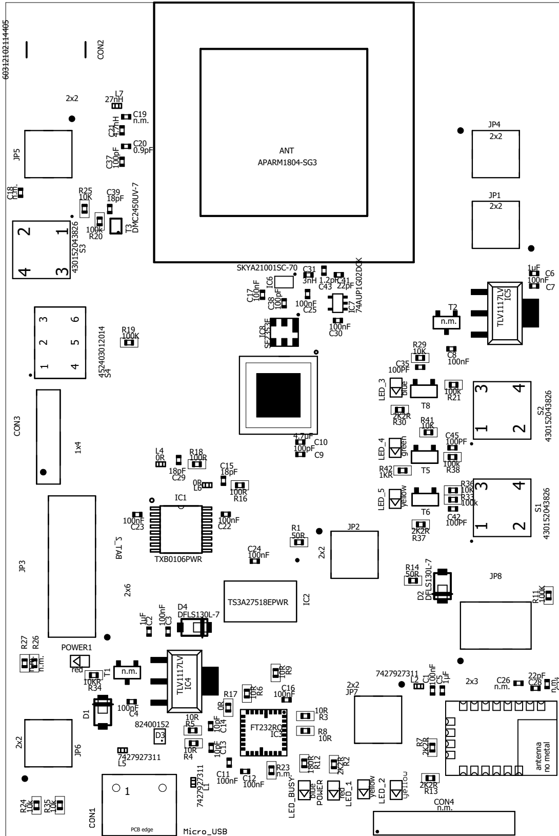
Figure 10: Assembly diagram
