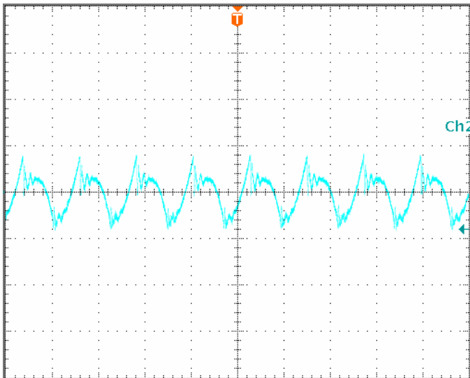
Figure 14: Output voltage ripple at nominal input voltage and max load current (20 mV/div, 2 µs/div). Load capacitance: 1\mu\text{F} ceramic capacitor and 10\mu\text{F} tantalum capacitor. Bandwidth: 20 MHz.
