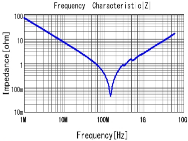
■ GRT1885C1H222JA02 |Z| DCOV, 25degC
