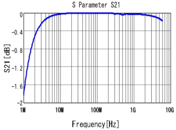
■ GRT1885C1H222JA02 S21 DCOV, 25degC
