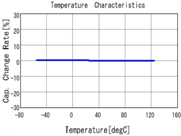
■ GRT1885C1H222JA02 C-Temp. capchange, DCOV, AC1Vrms
