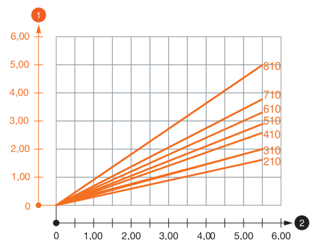
Belastingsdiagram console type AS 55
